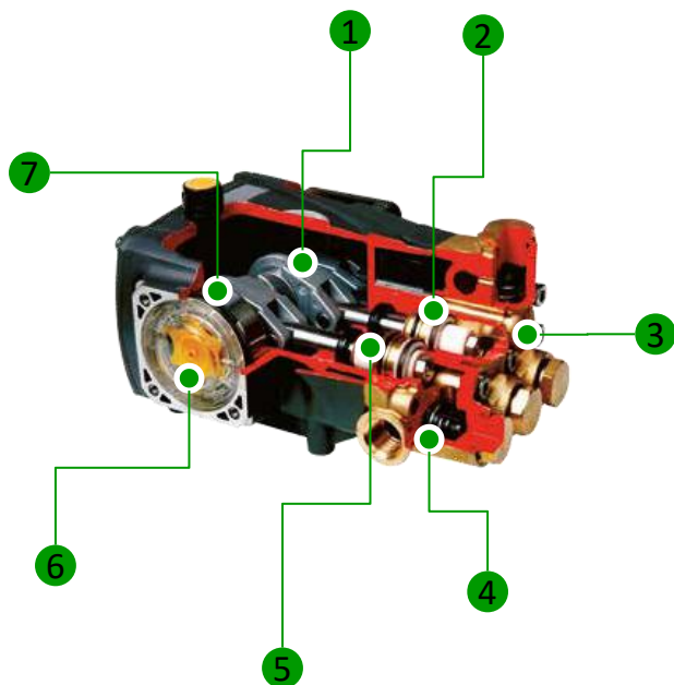
STB PUMP
